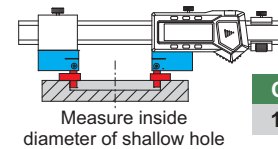
Measure inside diameter of shallow hole
